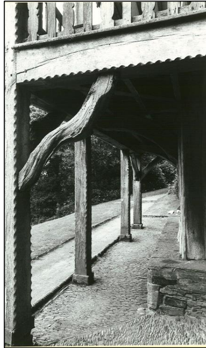
The ground floor timber supports to the veranda, and the pathway made of vertically laid pebbles.
